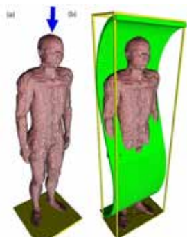
Figure D11 — Example 1: Human model exposed to an electromagnetic field reflected back into region occupied by the human. This region is shown as a yellow box. The standing wave is shown in green.
